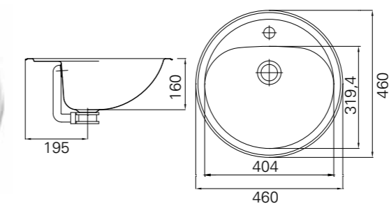
RRS901 NRRS-R02 Nedfellingservant i rustfritt stål 18/10 GTIN 7055570015612
