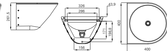
Endura ED3R Servant i rfr. stål 18/10 NRF 6175397 GTIN 7055570014394
