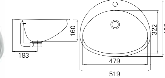
RRS902 NORS-R02 Nedfellingservant i rustfritt stål 18/10 GTIN 7055570015629
