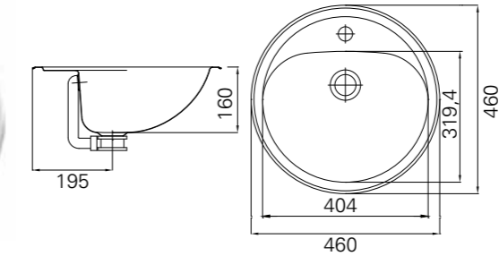
RRS901 NRRS-R02 Nedfellingservant i rustfritt stål 18/10 GTIN 7055570015612
