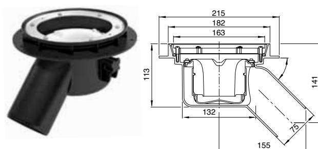
Undermontert
