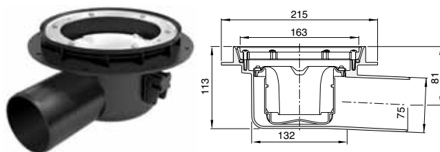
Undermontert
