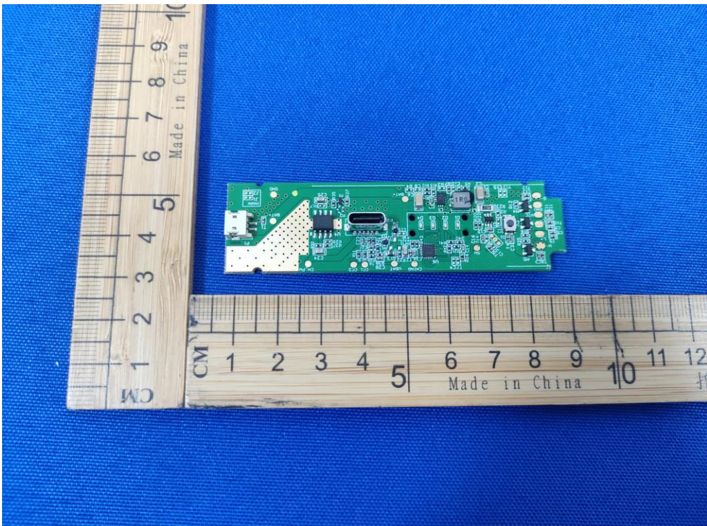
Figure 10. Top view of PCB
