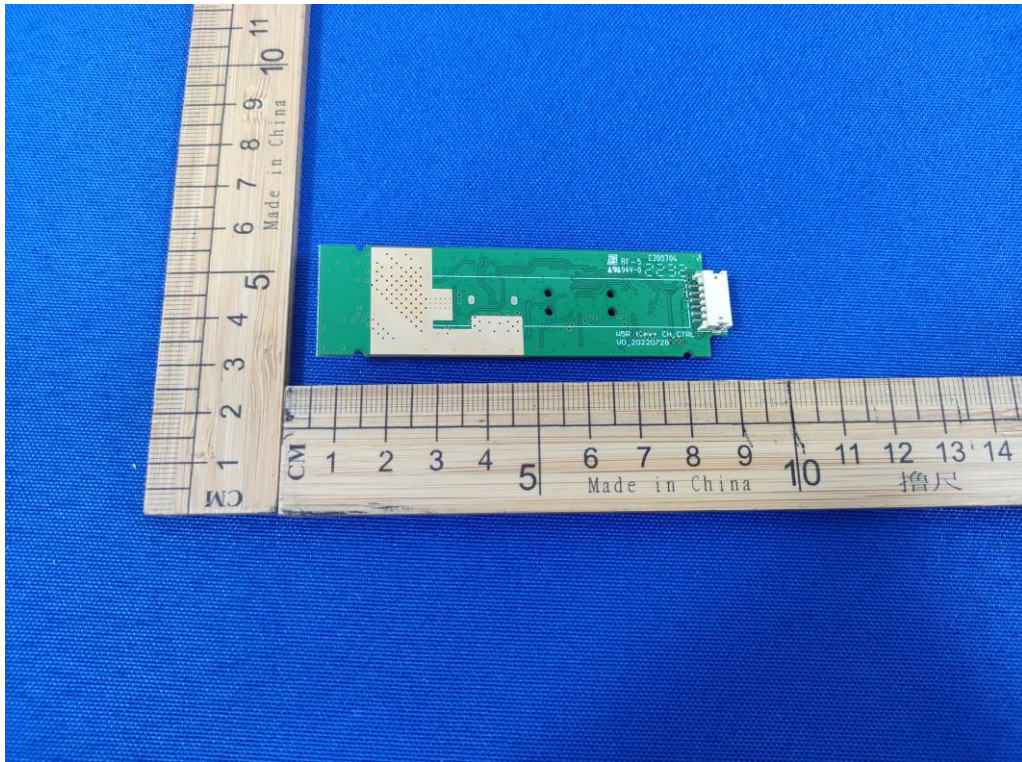
Figure 11. Bottom view of PCB
