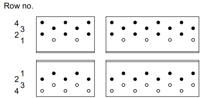
Nailing pattern 2
