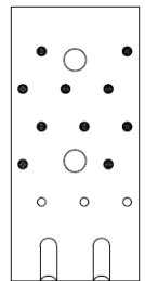
Nailing pattern 5
