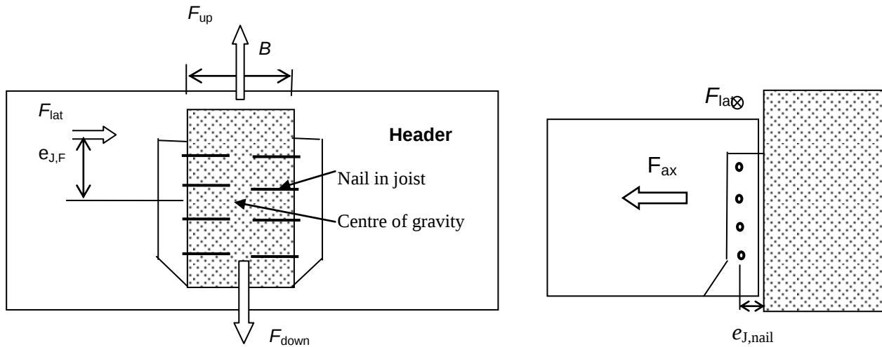
Figure 1: Definition of F_{\text{down}} , F_{\text{up}} , F_{\text{lat}} , F_{\text{ax}} , e_{j,F} and e_{j,nail}
