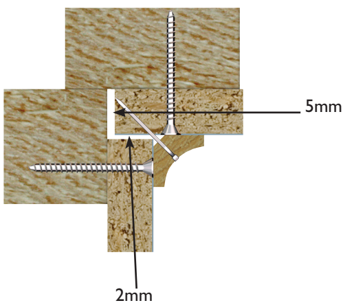
Fig. 3 - Clearance
