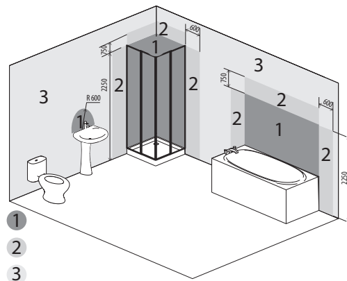
Bathroom zones
