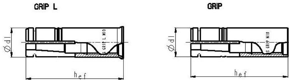
Expansion sleeve - 1
