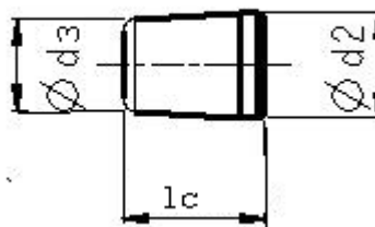
Tapered expansion plug - 2
