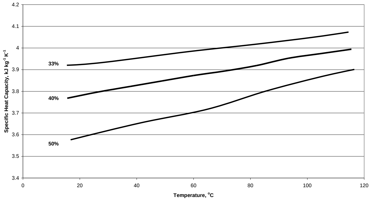
Specific Heat Capacity Chart
