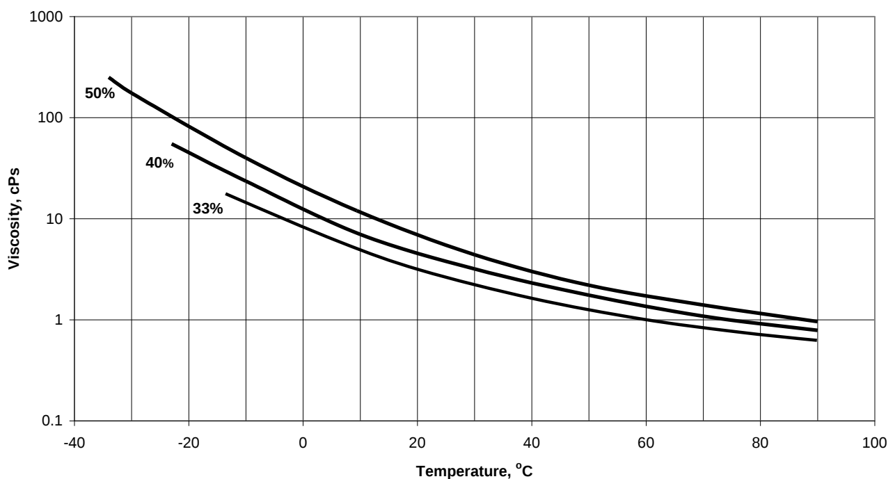
Viscosity Chart
