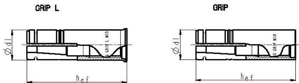
Expansion sleeve - 1
