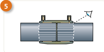
Stab pipe completely into fitting
