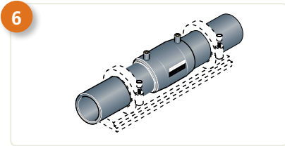
Align and clamp pipe
