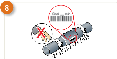
Do not disturb joint during cooling time
