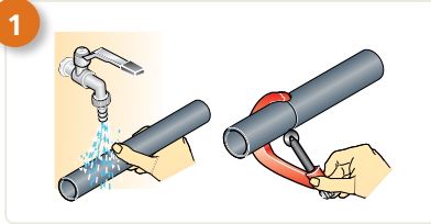
Clean pipe and cut ends squarely
