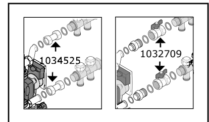
Uponor Vario B manifold
