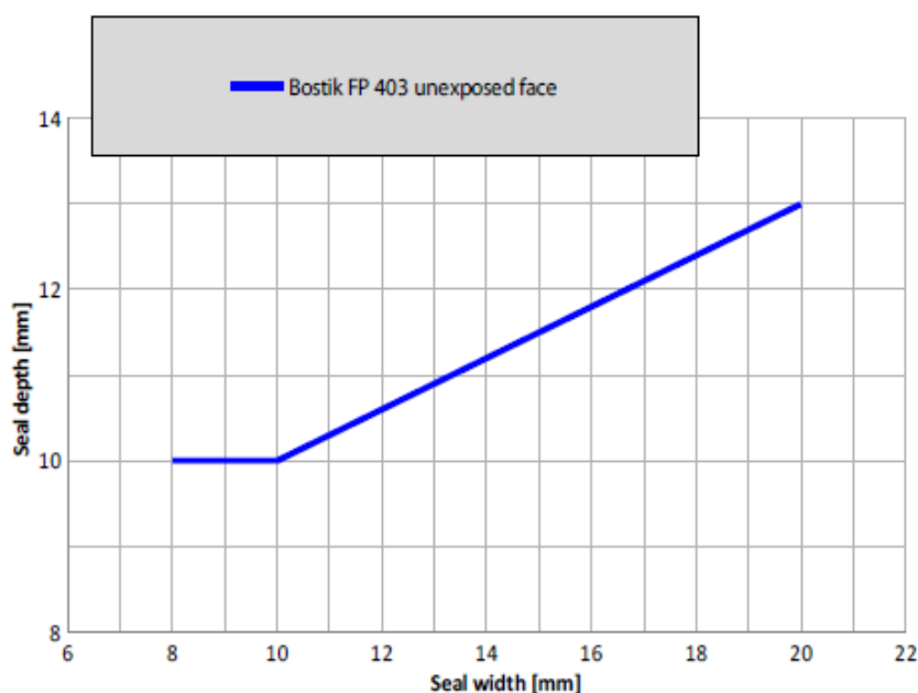
Graph 2: Minimum seal depth in relation to the seal width
