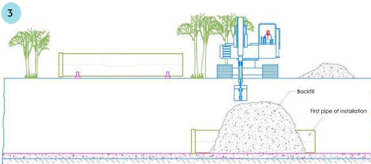
3- Fix the first pipe with backfill material.
