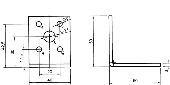
Figure B. 21 Dimensions of Angle Bracket 631 200 20
