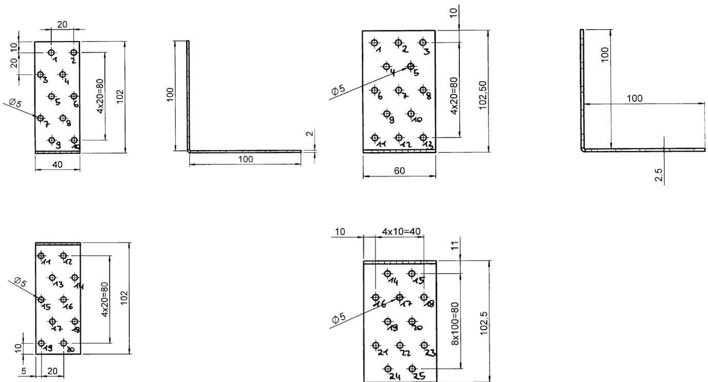
Figure B. 51 Dimensions of Angle Bracket 631 140 20
