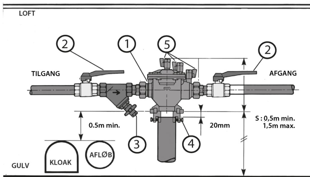
Fig. Installationstegning
