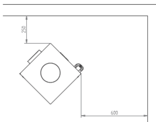
Distance to combustibles without insulated flues
