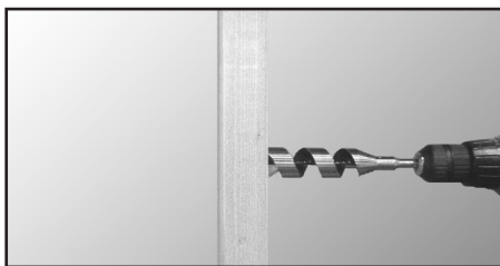
Bor 32mm hull i stender.
