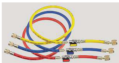
CCL-36-CA-1/2"-20UNF
