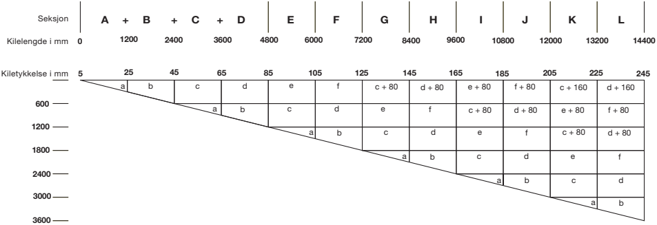
TF-takkiler
