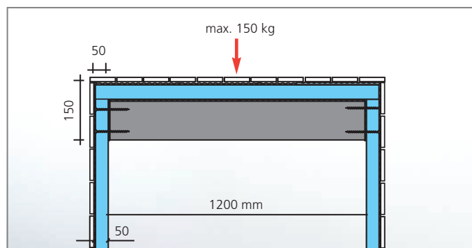
Load-bearing capacity.
