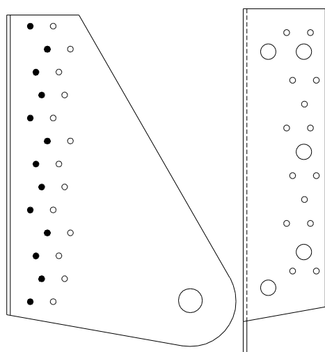
Timber width: b \geq 58 13 CNA4,0xl connector nails in face of connector
