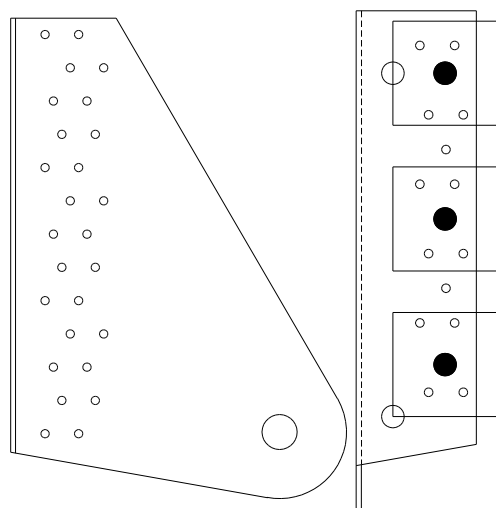
Timber width: b \geq 58 3 M12 bolts with washer in edge flap of connector
