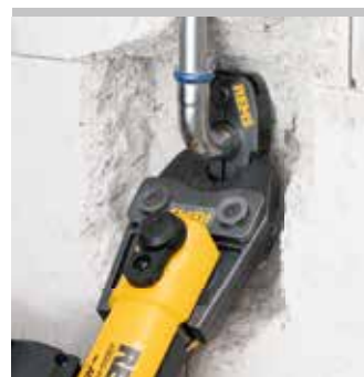
REMS pressring 45° (PR-2B) Patent EP 2 774 725
