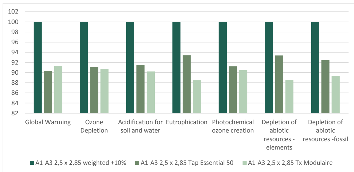
Figure 1: Comparison between Tapiflex/TX product and the average one (surface density between 2.5 and 2.85 kg/m 2 )
