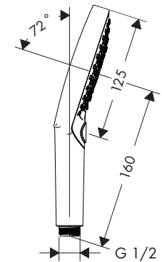
Raindance Select S 120 3jet PowderRain 26014000
