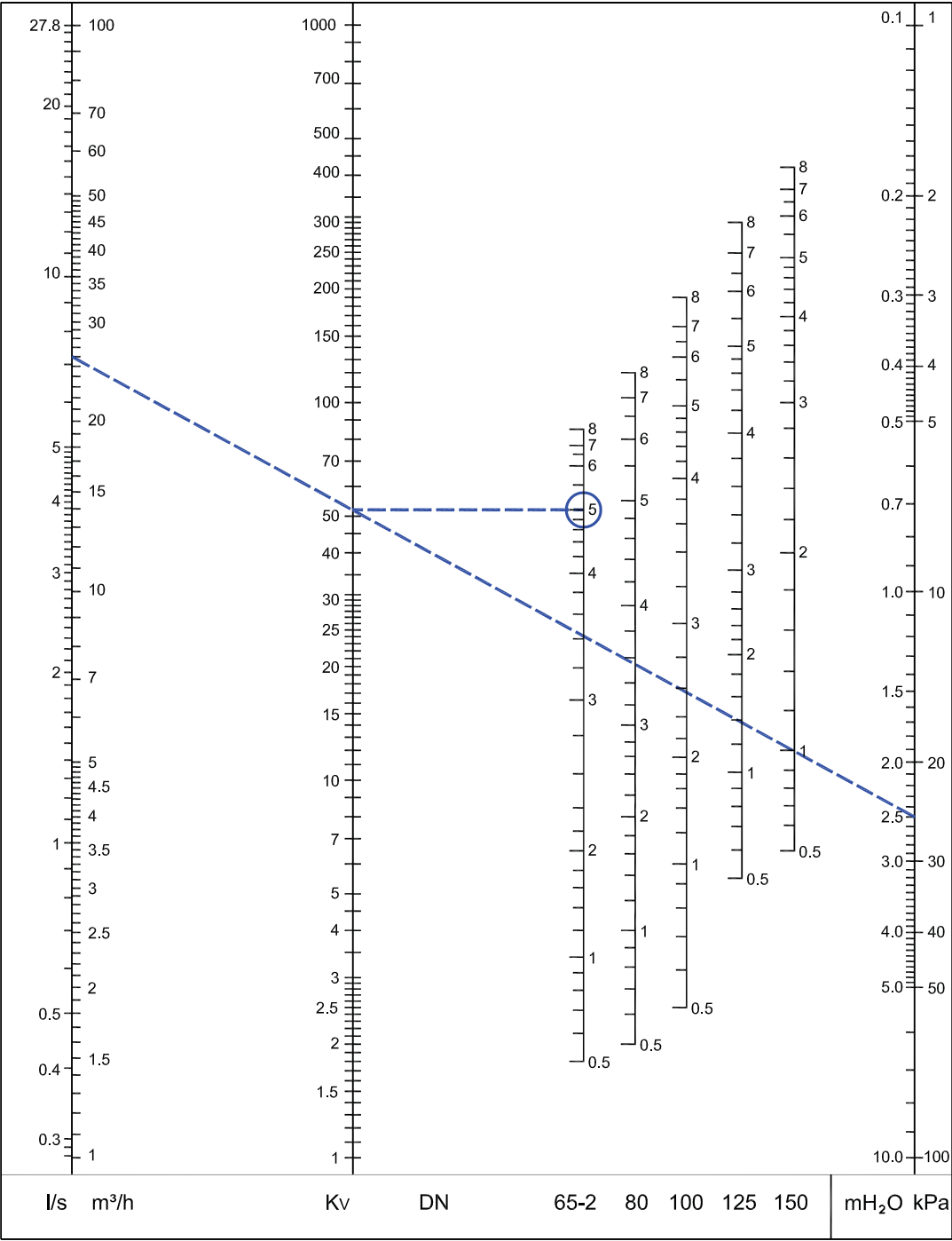
Diagram DN 65-150
