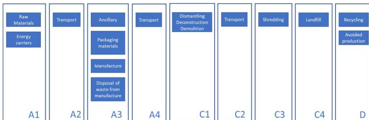
Figure 2: System boundaries for the study of the aluminium profiles Hydro Extrusion Sweden AB.
