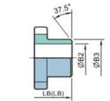
LB (Butt-welding End) LE (Extended Butt-welding End)
