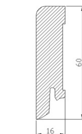
Fotlist 60x16 mm
