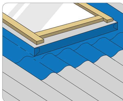
Takvindu/solcellepanel
