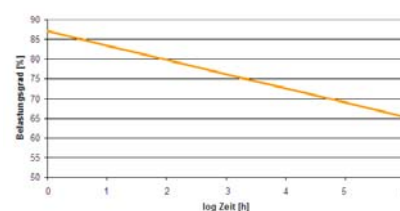
Figure 2: Creep rupture curve for Miragrid GX geogrids
