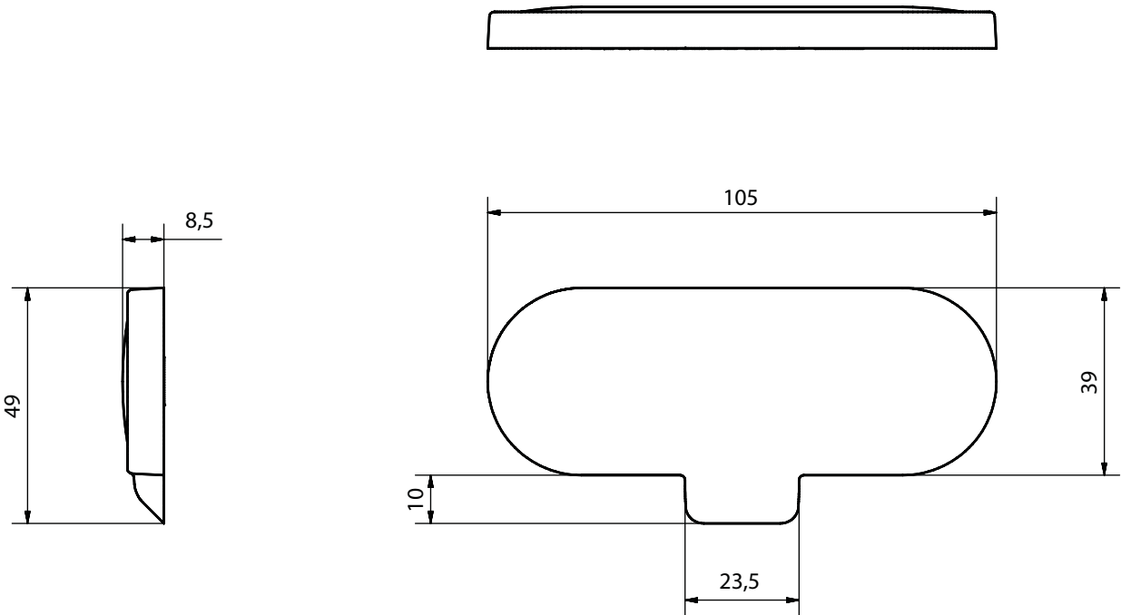
LK ArcTennaOnWall
