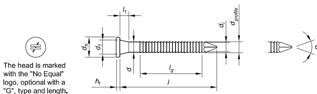
Drawing 1: CNA Connector nails
