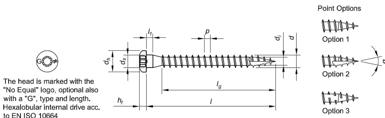
Drawing 2: CSA Connector screw
