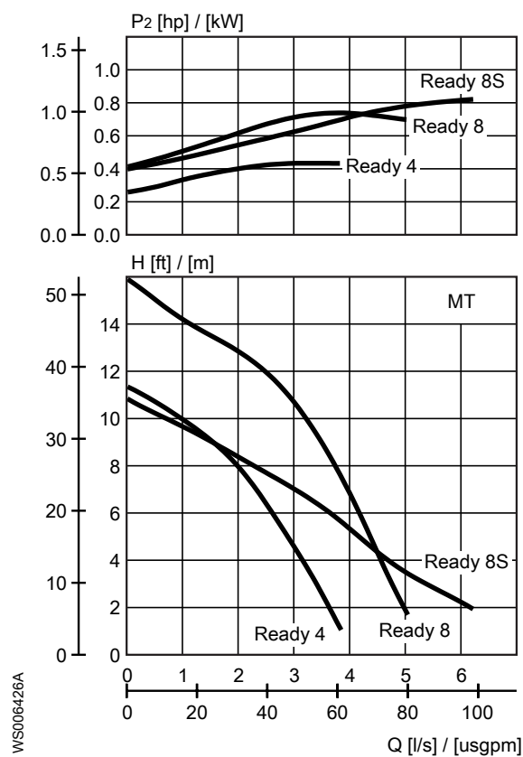
Figur 5: 60 Hz
