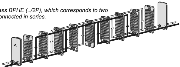
Dual-over-Two-Pass BPHE (.../D2P)
