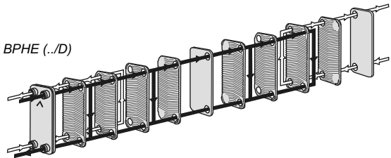
Two-Pass BPHE (./2P), which corresponds to two units connected in series.
