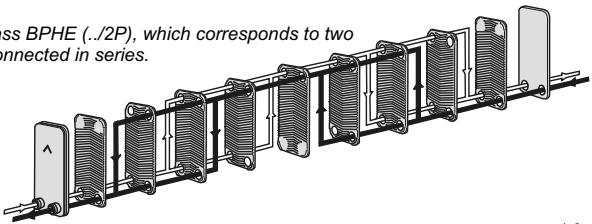
Dual-over-Two-Pass BPHE (./D2P)
