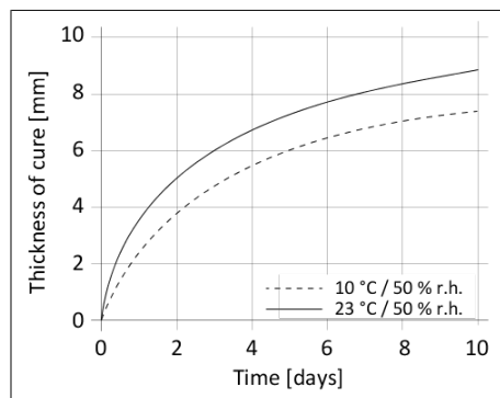
Diagram 1: Herdehastighet for Sikaflex®-292i
