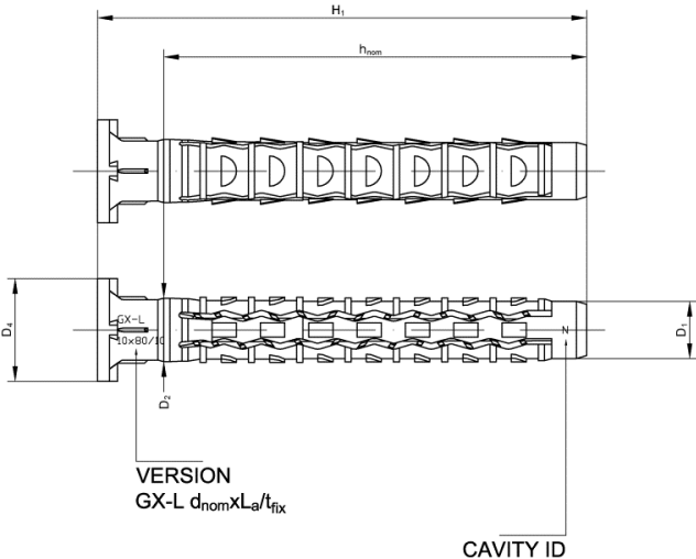
Version with collar for size \phi 10 only
