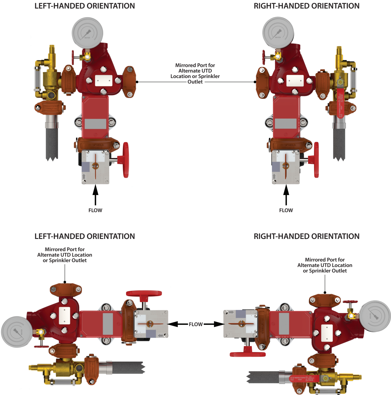
REPRESENTATIVE OF 1¼ - 6-INCH/42.4 - 168.3-MM SIZES (3-INCH/88.9-MM SIZE SHOWN)
