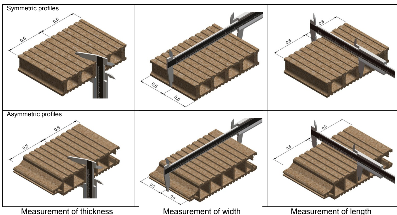
Figure 5: Measuring points for the determination of swelling characteristics.
