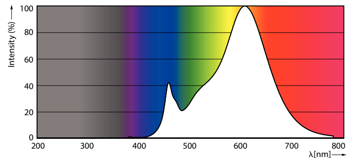
LEDcapsule LV 2,1W G4 827
