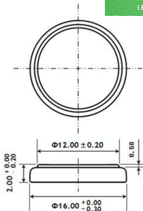
Dimension Drawing
