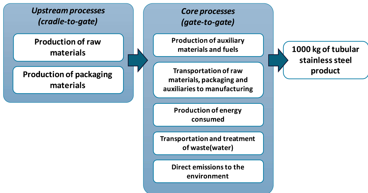
Figure 1. System diagram.
