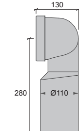
C + K3 WC - Stos, Universal, 110 muff RSK 310 66 87
