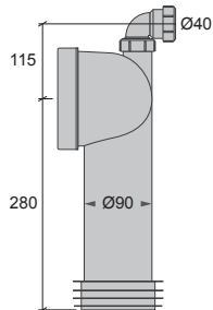
A + K3 WC - Stos, Universal X-tra RSK 310 66 61 NRF 619 66 74
