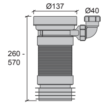
A WC - Stos, X-tra Flexibel RSK 310 67 28
