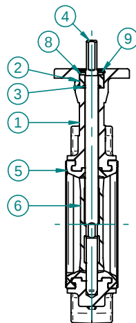
DN 50/100
