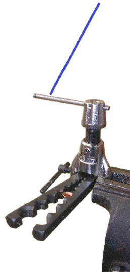
Easy bench-vice fixing
