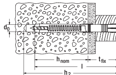
FUR-T - with fisher countersunk head safety screw
