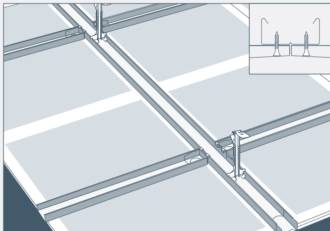
Opphengssystem. GK - system
