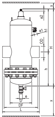
SPIROCOMBI DEMONTERBAR HI-FLOW FOR SVEISING
