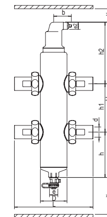
SPIROCROSS MESSING
