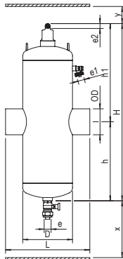
SPIROCOMBI HI-FLOW FOR SVEISING
