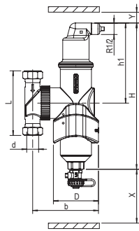
SPIROCOMBI MB3
