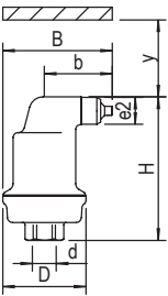
SPIROTOP SOLAR
