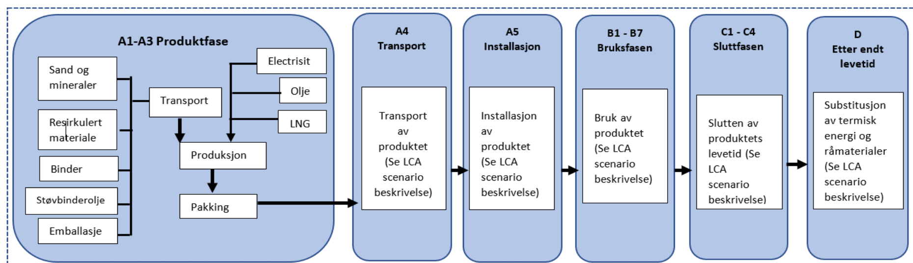
Figur 1: Systemgrense
